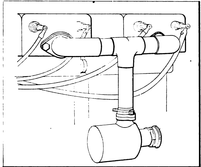
Fig. 12—Make-up manifold showing right-angle turns, involving a raiser and two branches.
